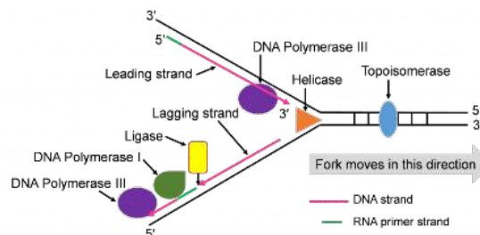
Figure 10e. Ligase must form a sugar-phosphate bond between the last nucleotide placed by DNA pol I and the first nucleotide placed by DNA pol III. Image by Walter Suza.
