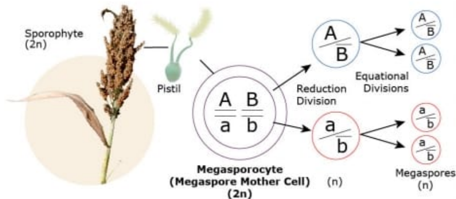
Figure 13 Megasporogenesis process. Photo by Iowa State University.
