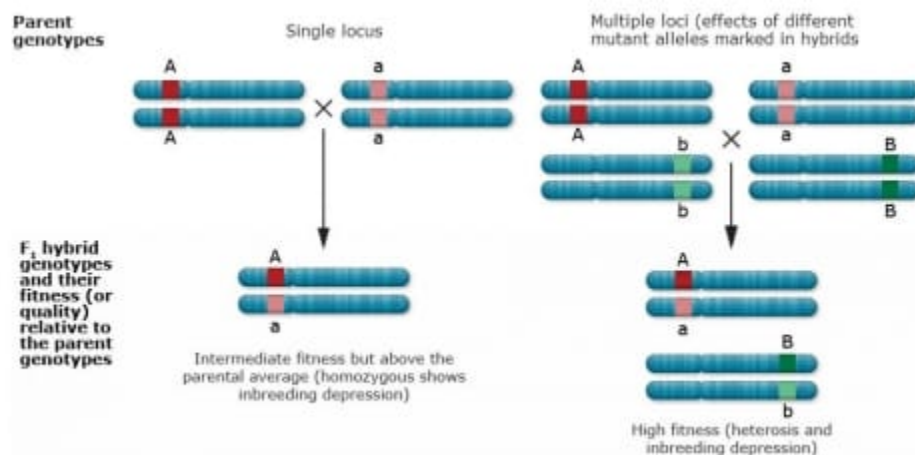
Figure 6 Dominance hypothesis. Summary of the main genetic hypotheses for inbreeding depression and heterosis. Adapted from Charlesworth and Willis, 2009.
