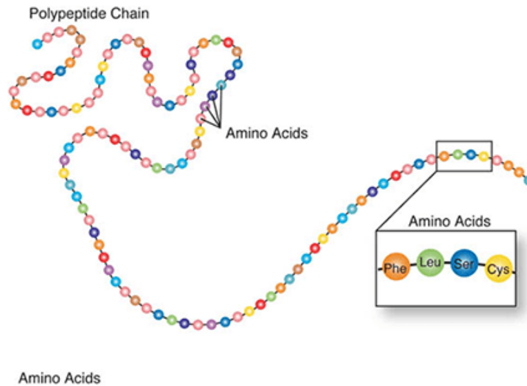
Figure 18 Amino acids bond together with peptide bonds to form long chains of polypeptides. Illustration from NIH-NHGRI, 2011.
