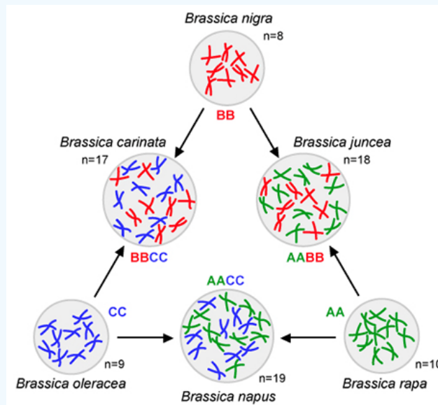
Figure 3 The “Triangle of U”: evolution and relationships among Brassica species. Adapted from U, 1935.
