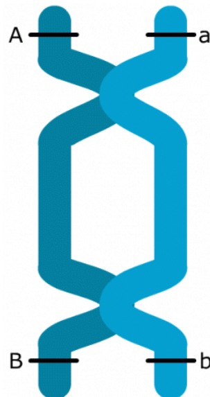
Figure 13 Double crossover event.
