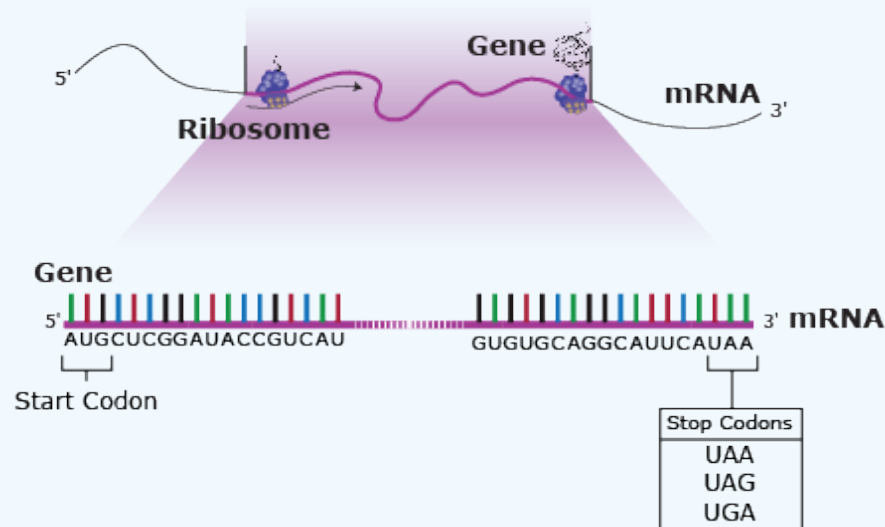
Figure 22 Stop codons signal a halt to protein synthesis. Illustration from NIH-NHGRI, 2011.
