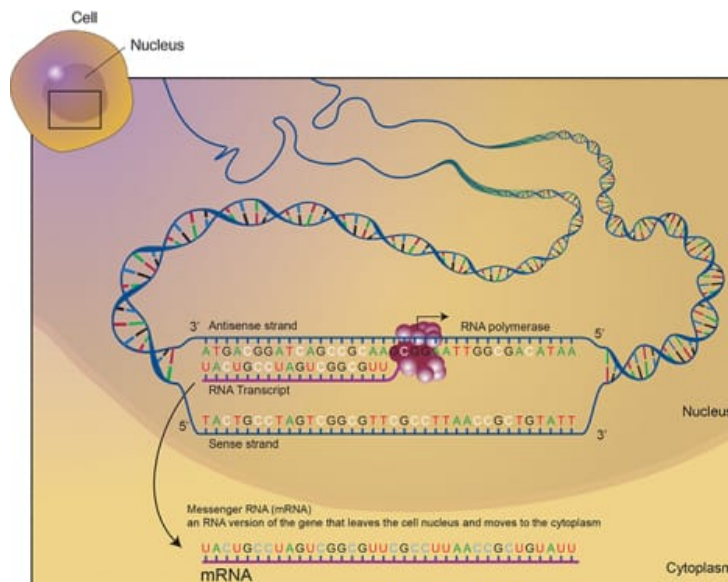
Figure 12 Messenger RNA(mRNA) is a single-stranded RNA molecule that is complimentary to the coding regions (exons) of one of the DNA strands of the gene. Illustration from NIH-NHGRI, 2011.
