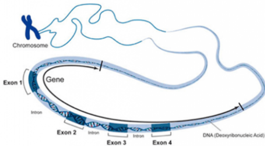
Figure 11 During RNA processing, the non-coding DNA sequences of the gene known as introns are removed and genetic information in exons is encoded. Illustration from NIH-NHGRI, 2011.
