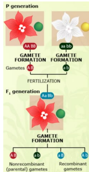
Figure 3 Formation of gametes with parental (left side) and non-parental (recombinant; right side) allele combinations at the two loci A and B.
