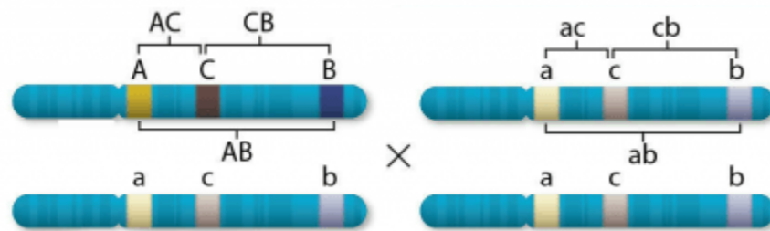
Figure 12 Example for a testcross (backcross) as a first step toward a three-point analysis. Adapted from Russell, 2010.
