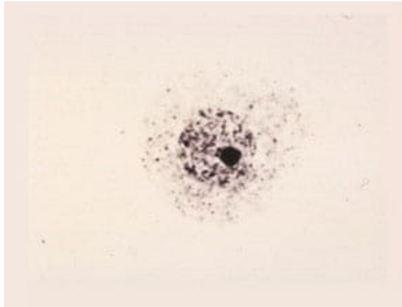
Figure 49 Early Uninucleate Cell.
