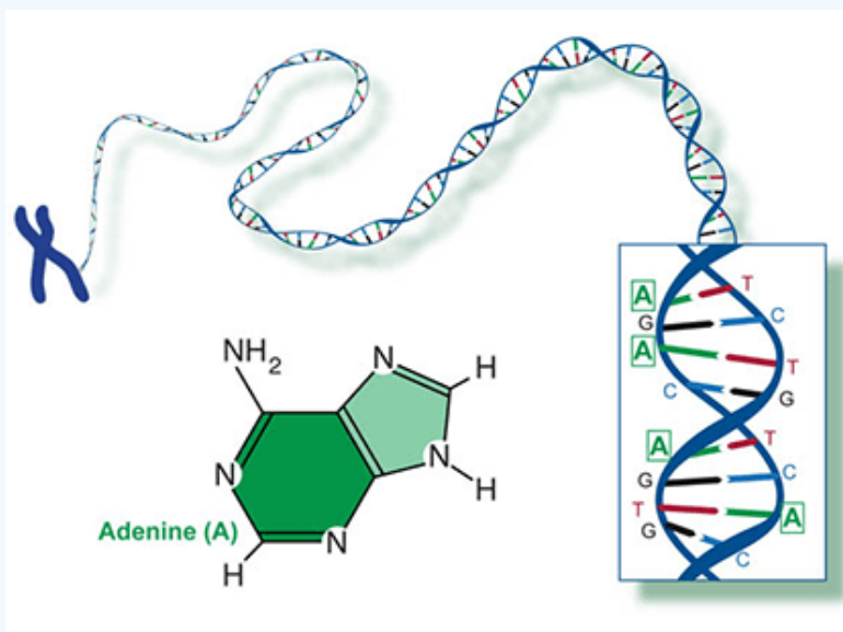
Figure 13 Adenine, a nitrogenous base in DNA and RNA, is a type of purine. Illustration from NIH-NHGRI, 2011.
