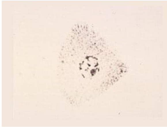
Figure 48 Free Cell from Quartet.
