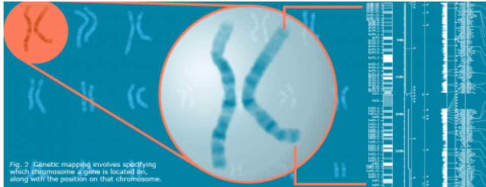
Figure 2 Genetic mapping involves specifying which chromosome a gene is located on, along with the position on that chromosome. Illustration by Iowa State University.
