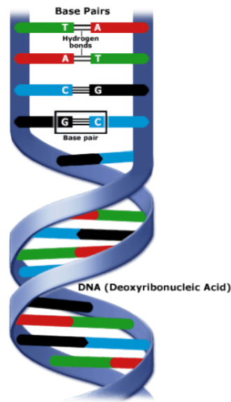
Figure 8 DNA molecules consist of two strands bound together by hydrogen bonds. Illustration from NIH-NHGRI, 2011
