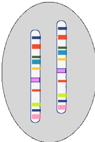
Figure 1 Nucleus with one pair of homologous chromosomes.
