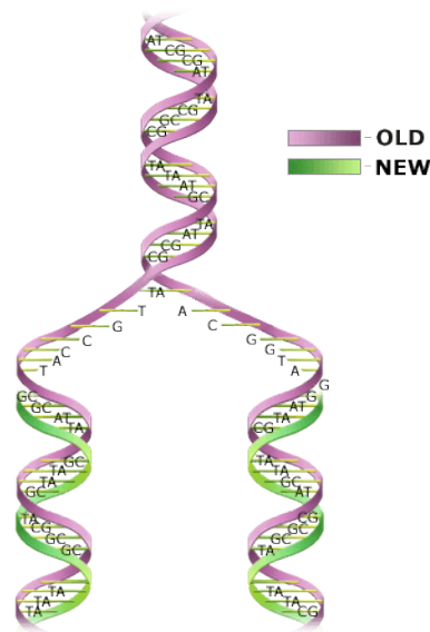
Figure 4 Semiconservative replication of DNA.
