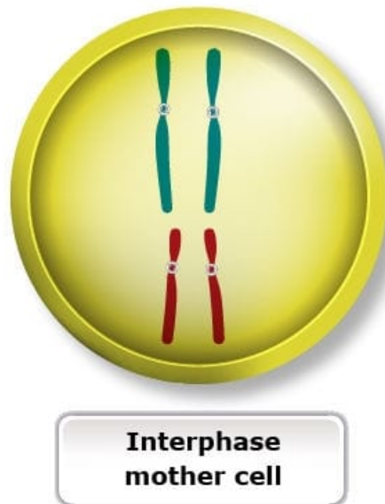
Figure 8 Interphase mother cell.
