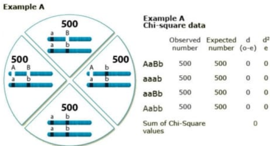
Figure 9 Example A. Expected vs. observed distributions of phenotypes
