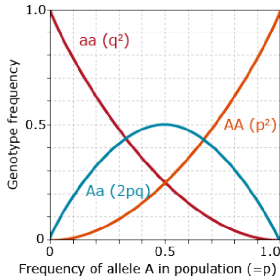
Figure 13 Relationship between genotype frequencies and gene frequency for two alleles in a population in Hardy-Weinberg equilibrium.
