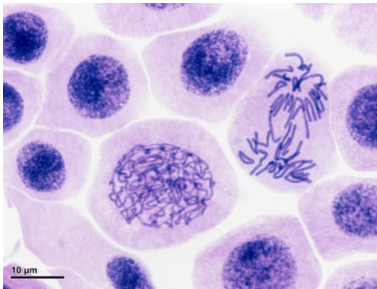
Figure 5 Onion cells stained to show contrast between the nucleus (dark) and the cytoplasm (lighter purple). Two cells at center are undergoing mitosis. Photo licensed under CC-BY-SA 2.0 via Wikimedia Commons.
